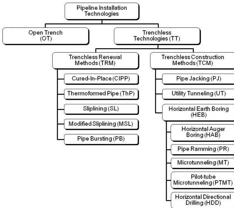
Figure 2.1. Underground pipeline installation methods.
