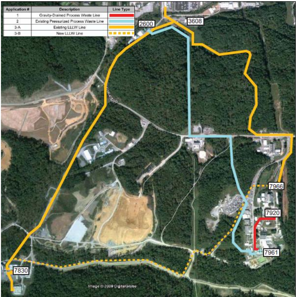
Figure 3.1. Select ORNL wastewater pipeline locations.
