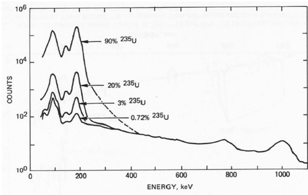
Figure 1 Response of a NaI detector to uranium in U_3O_8 with constant ^{238}U at various enrichments.
