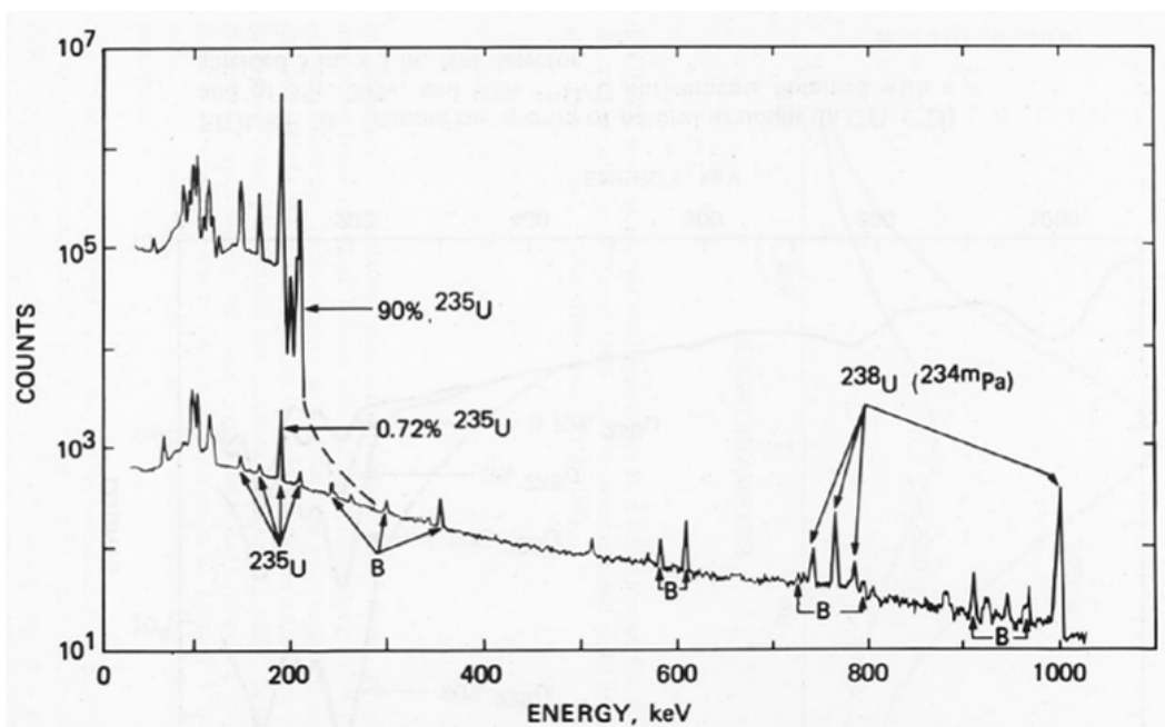
Figure 2 HPGe response to natural and enriched uranium in U_3O_8 with constant ^{238}U . 1
